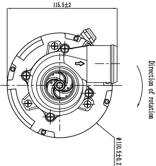
CQ28-28-46WA Water pump Technical conditions (技术条件)
